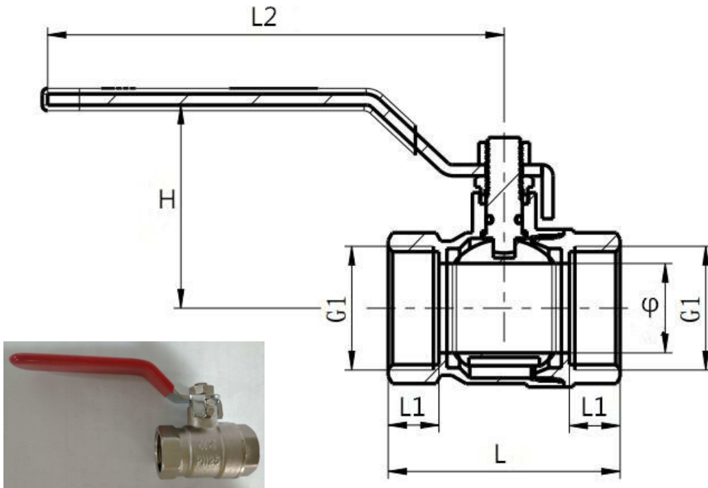
Brass ball valve FxF BSP threads, with steel handle Working temperature: Max. 110°C Working pressure: 25 bar
