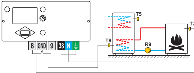
Picture 1 - D. h. w. storage tank
