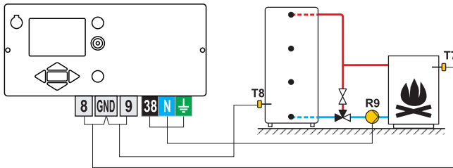
Picture 2 - Heat accumulator
