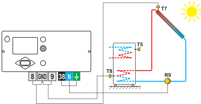
Picture 1 - D. h. w. storage tank
